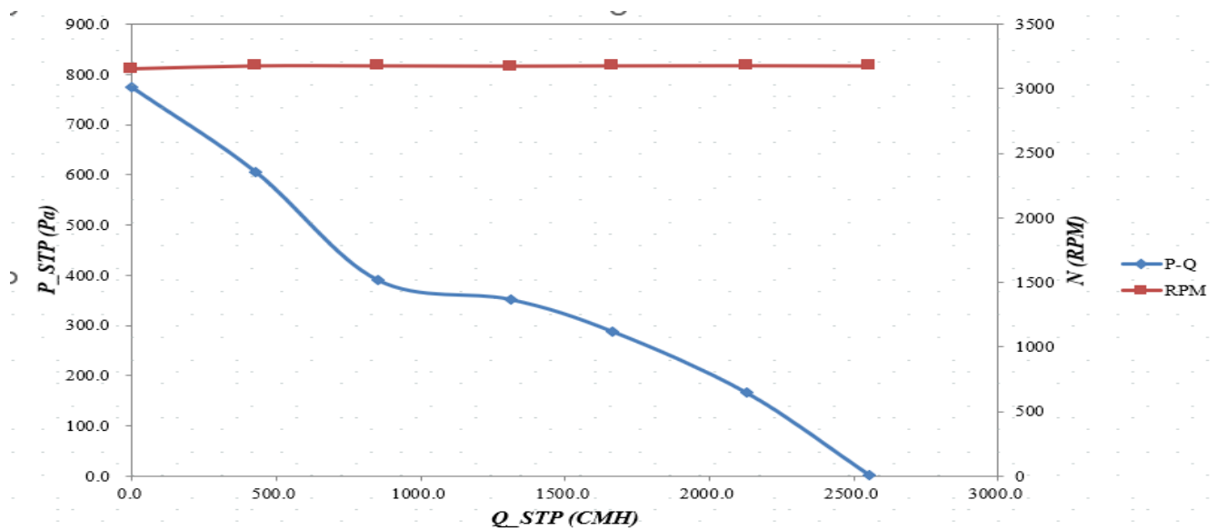
Performance Curve
